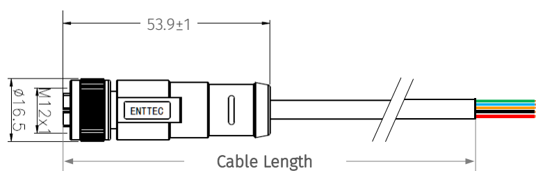
M12 Female Connector
